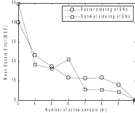
Fig. 2 (b) Average MSE for different cardinalities of randomly selected active sensor nodes..
